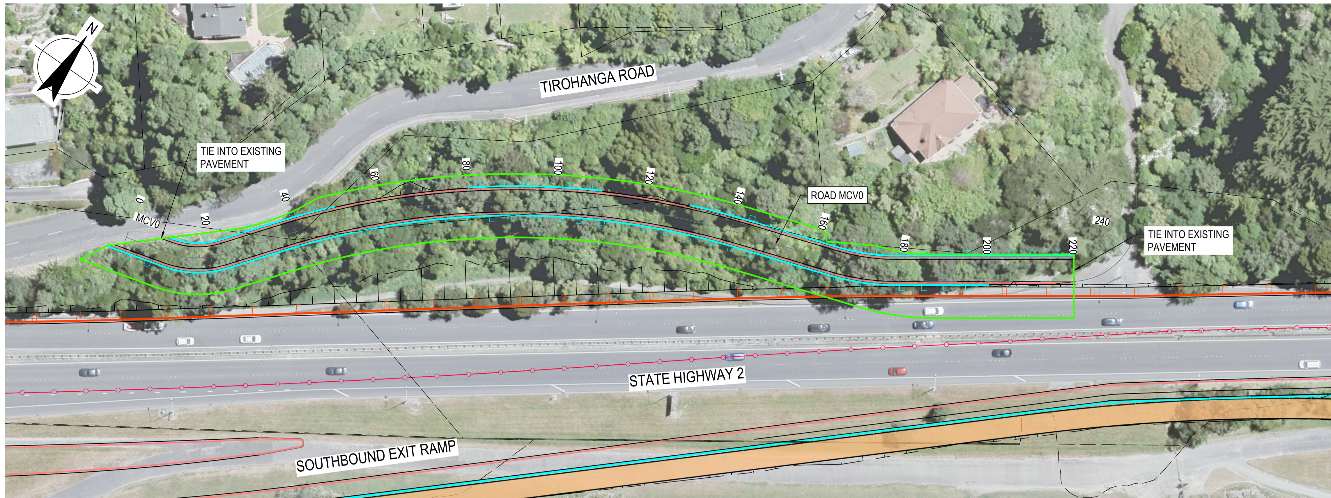
LAYOUT PLAN SCALE 1:500
